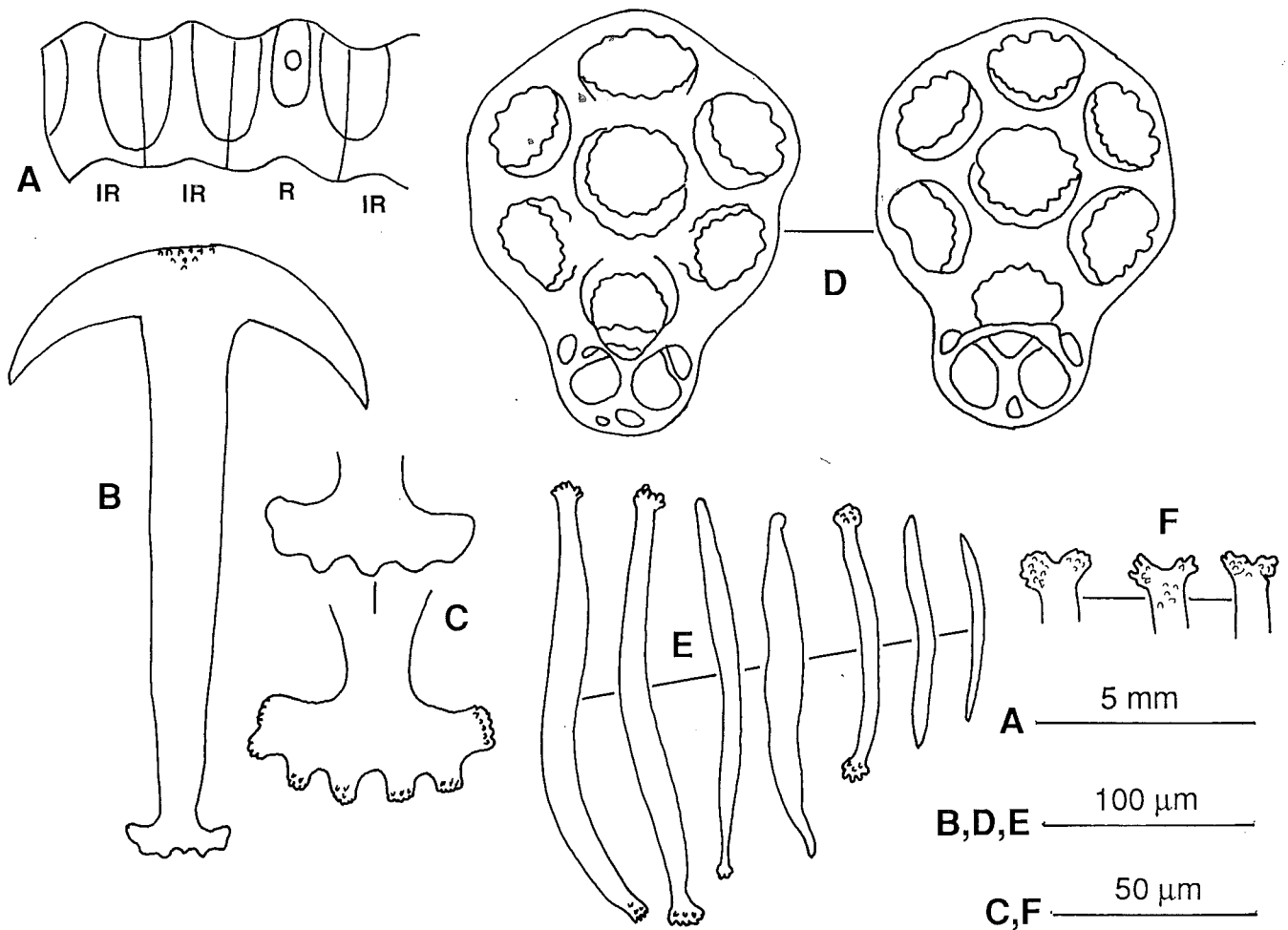
Fig. 11. — Euapta godeffroyi (SEMPER, 1868). A: calcareous ring (r: radial piece; ir: interradial piece); B: anchor; C: stocks of anchors; D: anchor-plates; E: rods of the tentacles; F: extremities of the tentacular rods.
