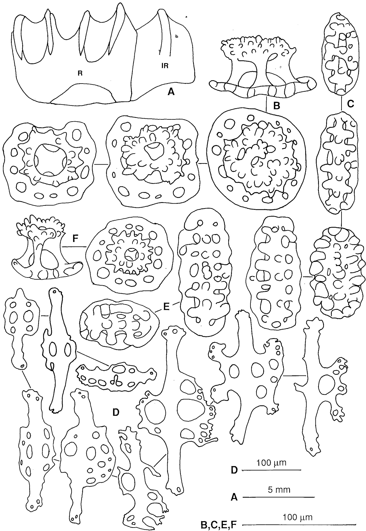
Fig. 1. - Holothuria (Microthele) nobilis (SELENKA, 1867). A: calcareous ring (r: radial piece; ir: interradial piece); B: tables of the dorsal body wall; C: buttons of the dorsal body wall; D: perforated rods of the dorsal papillae; E: buttons of the ventral body wall; F: tables of the ventral body wall.
