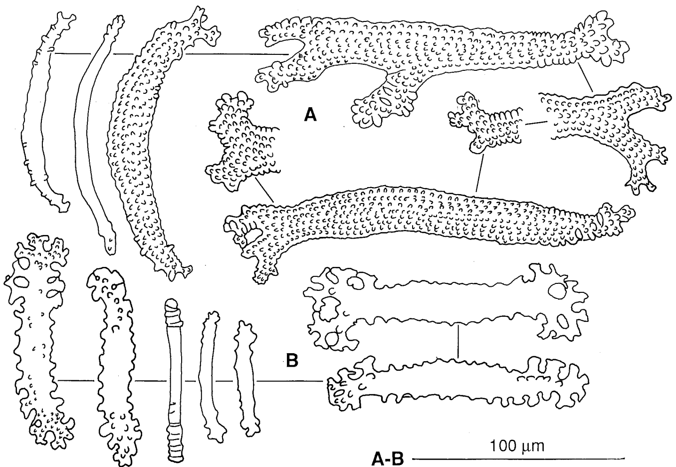
Fig. 6. — Holothuria (Semperothuria) cinerascens (BRANDT, 1835). A: rods of the dorsal tube feet; B: rods of the tentacles.
