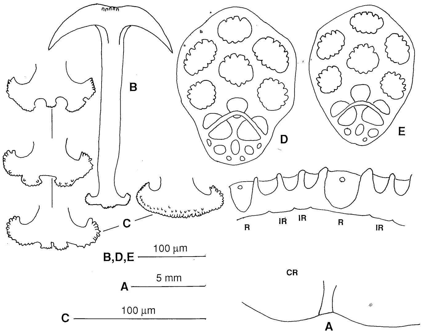
Fig. 12. — Polyplectana kefersteini (SELENKA, 1867). A: calcareous ring and cartilaginous ring (r: radial piece; ir: interradial piece; cr: cartilaginous ring); B: anchor; C: stocks of anchors; D: anchor-plate anteriorly located; E: anchor-plate posteriorly located.
