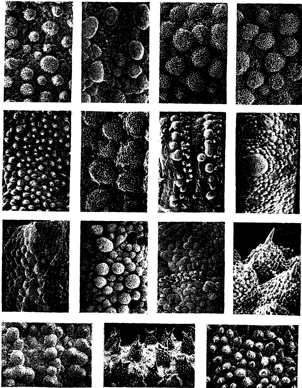
Fig. 28. Surface of disc (radial shield) and arms (basal dorsal, unless otherwise specified) of: top row, left to right, Astroboa granulatus , disc & arm; A. ernae , disc & arm; 2nd row, A. nigrofurcata , disc; A. nuda , disc; Gorgonocephalus dolichodactylus , arm, lateral; Astrochalcis tuberculatus , disc; 3rd row, Astroglymma sculptum , arm; Astrocladus ludwigi , disc & arm; A. tonganus , disc detail; bottom row, A. tonganus , arm; Astrocladus exiguus , disc detail & arm.
