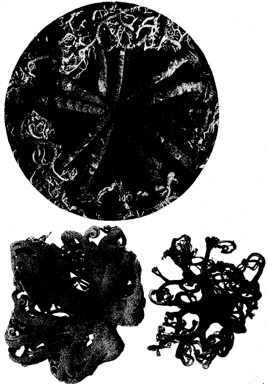
Fig. 22. Upper, Astroboa nuda , W of Carnarvon, W.A., 70.0 mm d.d. Lower left, Astrochalcis tuberculatus , Dampier, W.A., 17.0 mm d.d. Lower right, Astroboa granulatus , Lord Howe I., 11.0 mm d.d.
