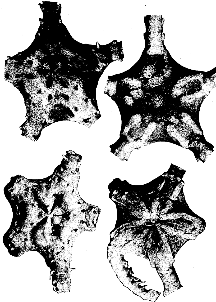
Fig. 3. Upper, Asteronyx loveni , juvenile (USNM 26173), 3.8 mm d.d. Lower, Astrodia tenuispina , syn-type of A. bispinosa Koe. (AM J3855), 7.5 mm d.d.
