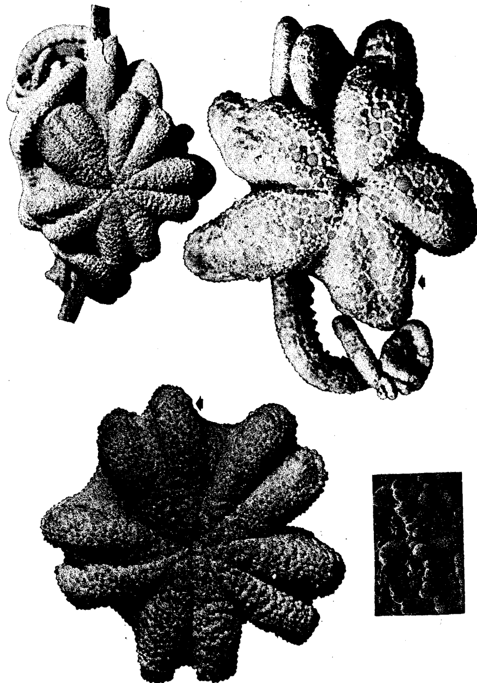
Fig. 10. Left, Asteromorpha (Astromoana) indicus , holotype (WAM 737.753), 10.0 mm d.d. Upper right, A. (Astromoana) reticulata , holotype (NZOI H254), 9.0 mm d.d. Lower right, A. reticulata , paratype (NMNZ Ech. 2878), 1.6-mm-long section of dorsal surface of arm. Arrows mark position of girdle band.
