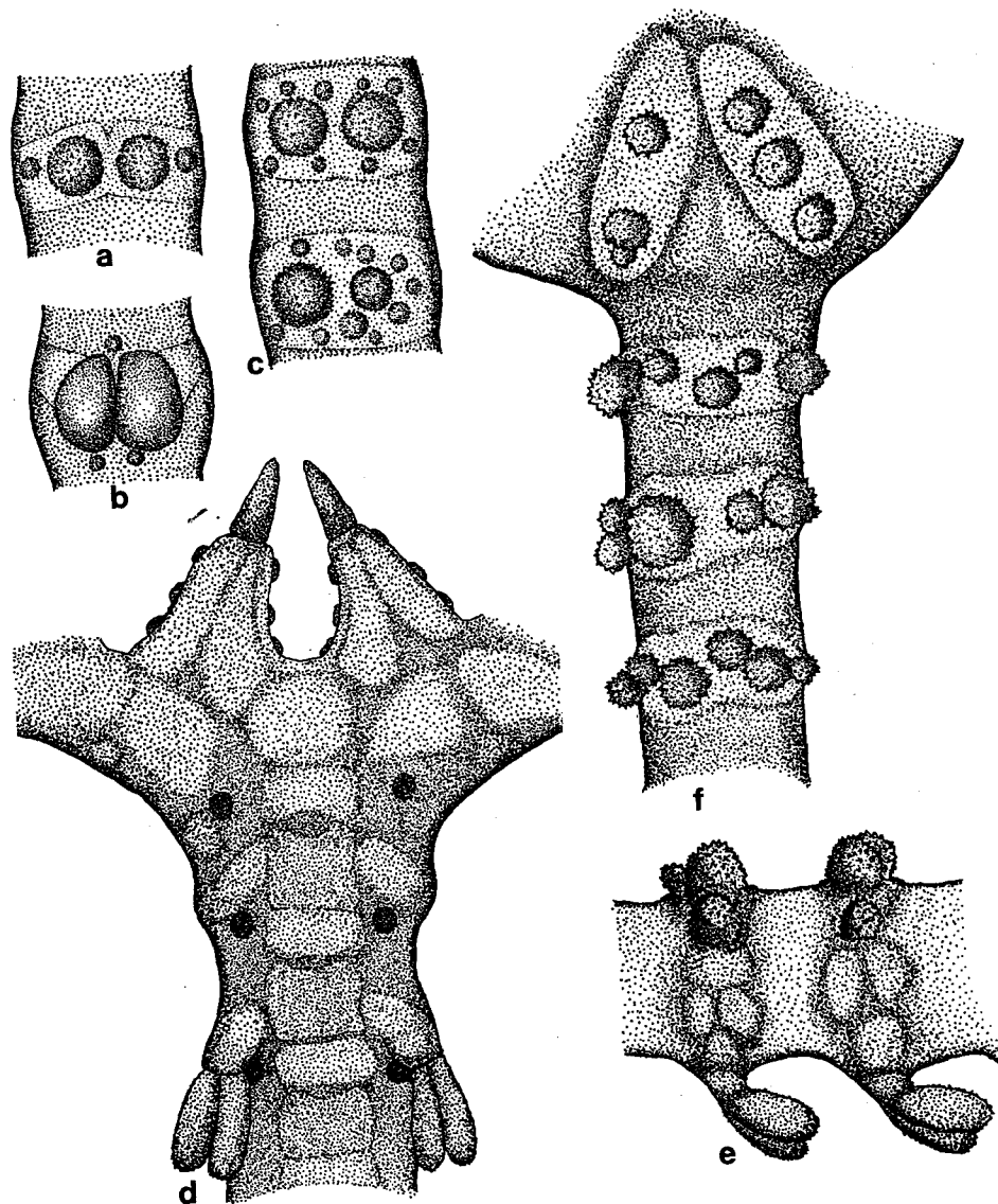
Fig. 27. a, d-f, Astroceras pleiades (holotype, AM J8503): (a) dorsal surface of distal arm segment; (d, f) ventral and dorsal views of arm base and adjoining disc; (e) lateral view of proximal arm segments. b, c, Astroceras nodosum (paratype, USNM E8695): (b) distal arm segment; (c) proximal arm segment.
