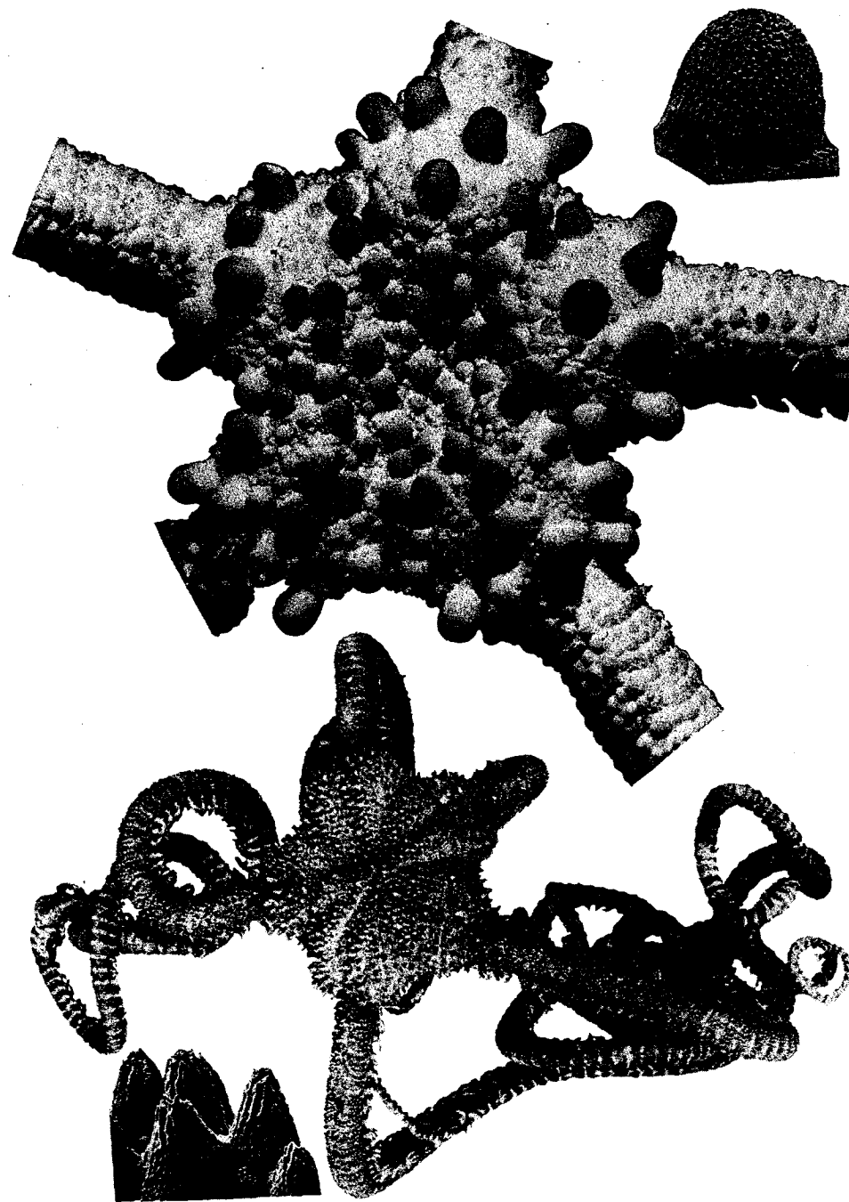
Fig. 9. Upper, Astrothrombus rugosus , Cuvier I., N.Z., 10.0 mm d.d. Lower, A. vecors , Bay of Plenty, N.Z., 14.0 mm d.d. Upper right & lower left, enlarged tubercles from inter-radial edge of oral frame (×21).
