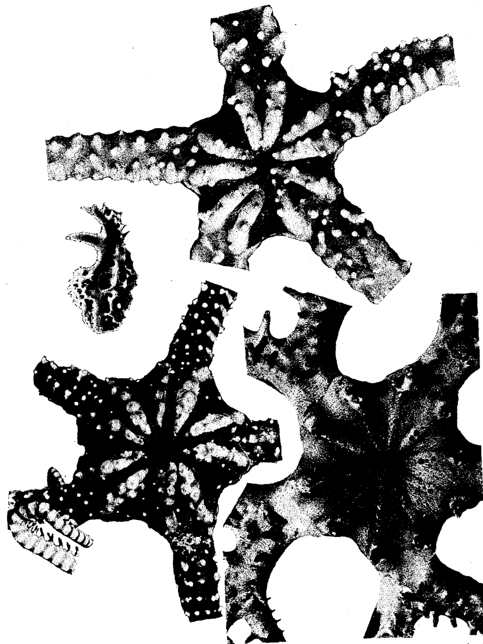
Fig. 25. Upper, Astroceras elegans , Three Kings Is, N.Z., 10.0 mm d.d. Middle left, distal arm-spine hooklet of A. pleiades , paratype (NMNZ, Ech. 1947), 0.24 mm long. Lower left, A. elegans , North Cape, N.Z., 14.0 mm d.d. Lower right, Euryale aspera , Bunbury, W.A., 24.0 mm d.d.
